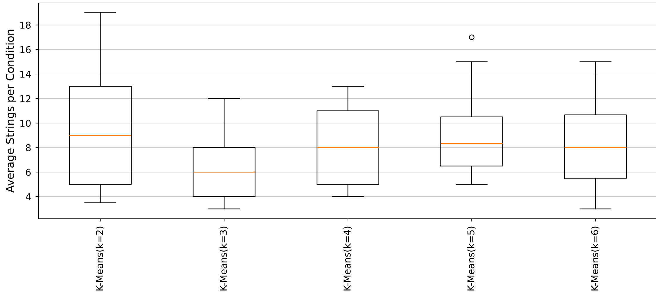
YARA Rules Average Strings per Condition Distribution (Cluster30_Size6 dataset)
